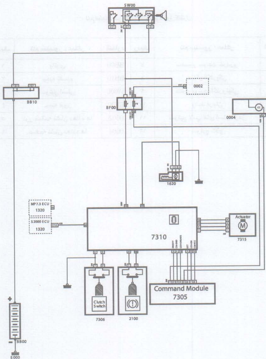
Cruise Control Schematic Diagram
